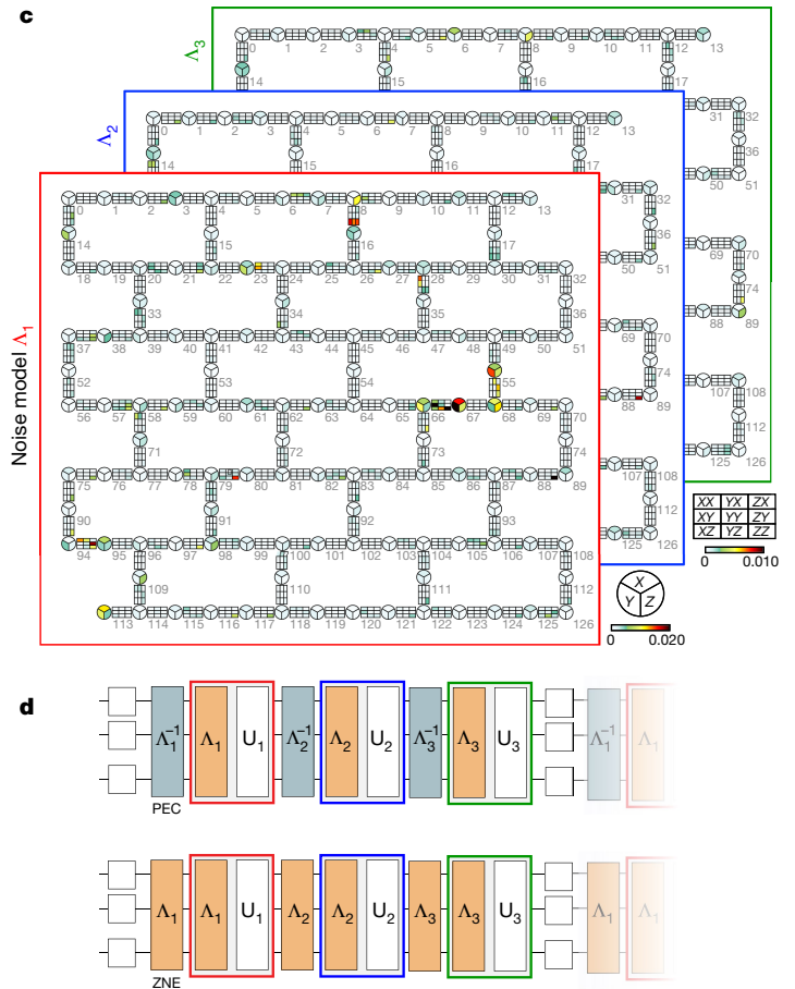
c , Characterization experiments efficiently learn the local Pauli error rates \Lambda_{li} (colour scales) comprising the overall Pauli channel \Lambda_i associated with the l th twirled CNOT layer. (Figure expanded in Supplementary Information IV.A). d , Pauli errors inserted at proportional rates can be used to either cancel (PEC) or amplify (ZNE) the intrinsic noise.
