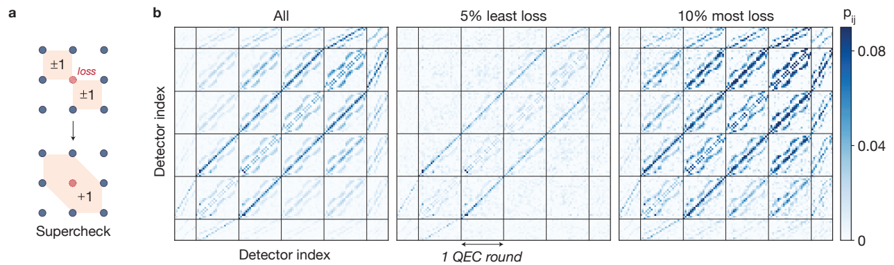
Extended Data Fig. 5. Characterizing effects of loss and leakage in repeated QEC. a , Superchecks. A lost data qubit results in anti-commuting stabilizers and a flickering error pattern. Producing stabilizers surrounding the lost qubit recovers commuting superchecks. b , Detection correlation p_{ij} matrix for five rounds of QEC on a d = 5 surface code. Data qubit errors appear as space-like correlations and ancilla measurement errors as time-like correlations between adjacent layers. Leakage results in additional persistent correlations between QEC rounds. By selecting shots with the fewest lost data qubits, these correlations are suppressed, indicating that leakage is dominated by loss which can be detected. Similarly, selecting shots with the most loss enhances the correlations.
